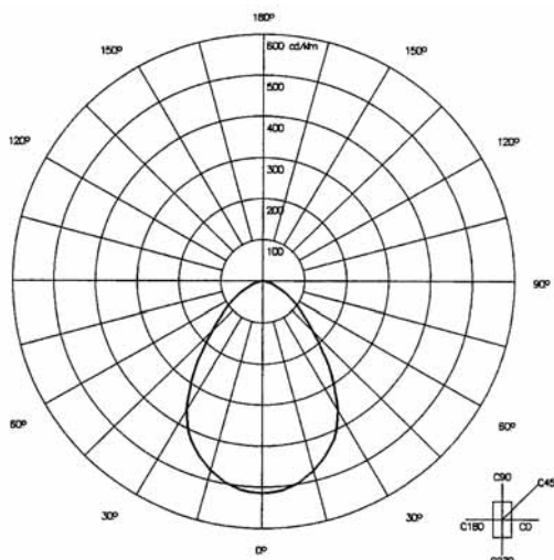
MBI 1000W
